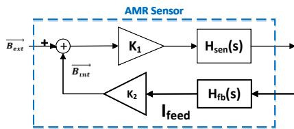
Fig. 2 Simplified analytic HMC-1001/2 sensor diagram.
