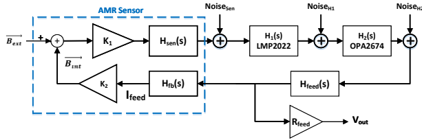
Fig. 4 Simplified analytic system diagram.
