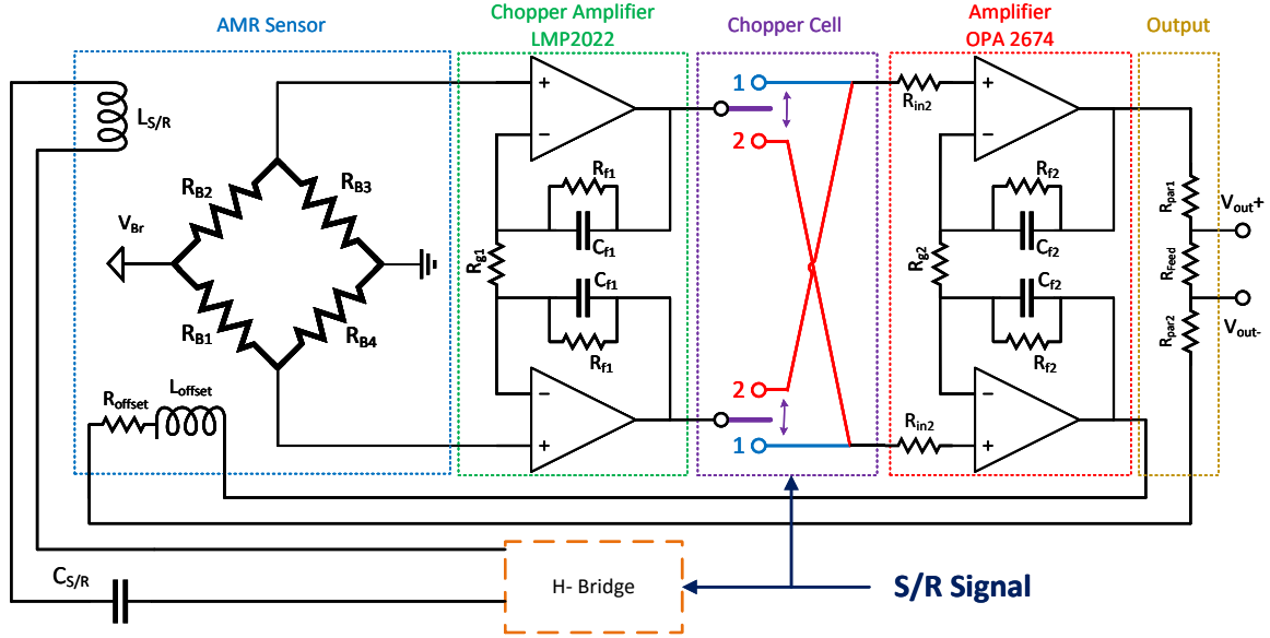
Fig. 1 The proposed closed loop architecture.
