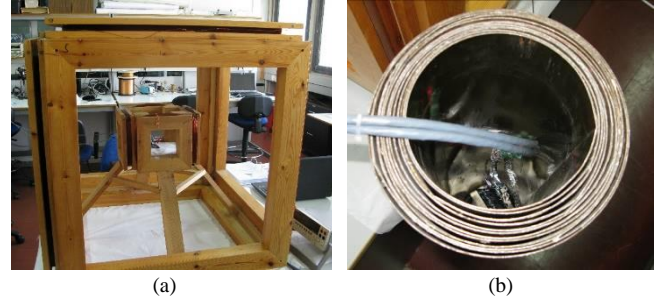
Fig. 5 Experimental setup, (a) cubic Helmholtz Coils (b) Magnetic Shield.
