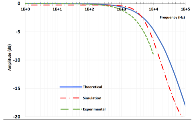
Fig. 8 AC Bandwidth Measurements.
