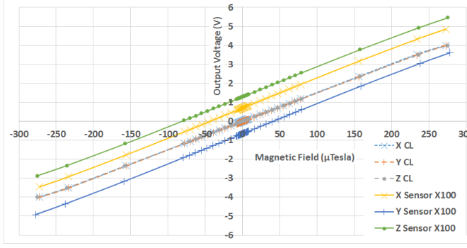
Fig. 6 DC Measurements.
