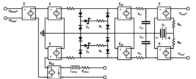
Fig. 3 Spice model for HMC-1001/2.
